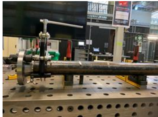
Figure 3.b: Side view of the flange-to-pipe alignment task with EZ-pipe-clamp holding flange to end of the pipe.
