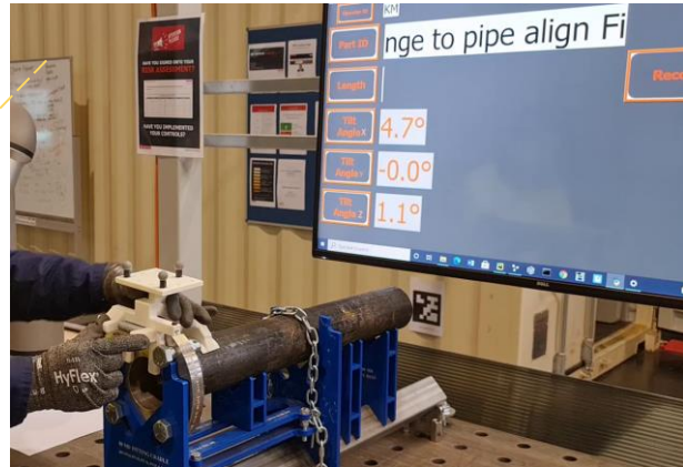
Figure 4.d: (i) Fit Rite pipe-fitting jig used for flange-to-pipe alignment; (ii) Harnessing digital spirit level for checking flange to pipe alignment. Digital spirit level angle data displayed on custom dimensional control GUI for OQE capture
