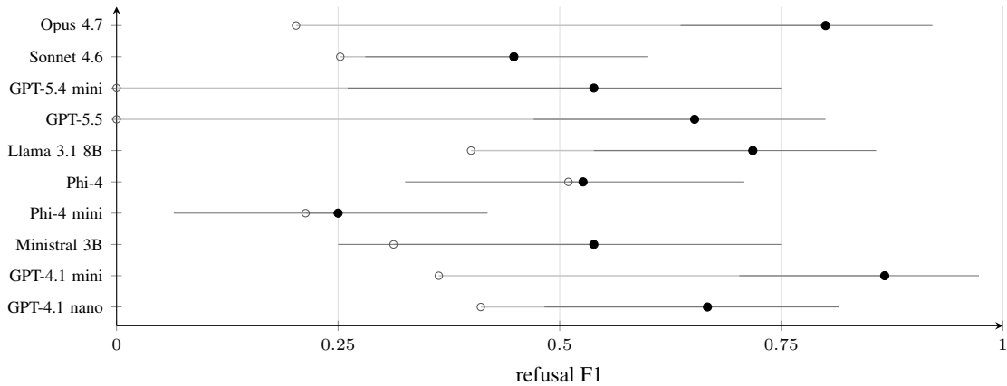
Figure 4: Refusal-F1 under model_only and sa_harness , per model. All 10 panel models improve under the harness; openai/gpt-4.1-mini reaches the highest harness F1 (0.867, CI [0.733, 0.967]).
