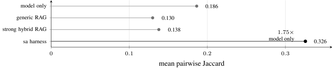
Figure 3: Mean pairwise Jaccard similarity of refused-item sets across 45 model pairs per condition. Only sa_harness increases agreement over model_only ; retrieval-only conditions slightly reduce mean Jaccard despite adding evidence.
